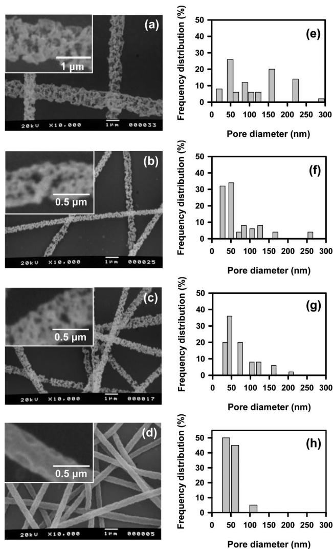
Figure 4. Scanning electron micrographs of the electrospun POM13 nanofibers from an HFIP solution at 75% relative humidity and pore size distributions as a function of electrical voltages: (a, e) for 4 kV, (b, f) for 6 kV, (c, g) for 10 kV, and (d, h) for 15 kV (tip-to-target distance = 10 cm).
