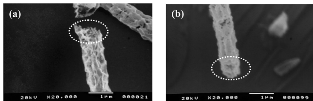
Figure 7. Scanning electron micrographs showing a cross section of POM13 nanofibers from an HFIP solution at 55% relative humidity, electrospun at (a) 4 kV and (b) 15 kV (tip-to-target distance = 10 cm).
