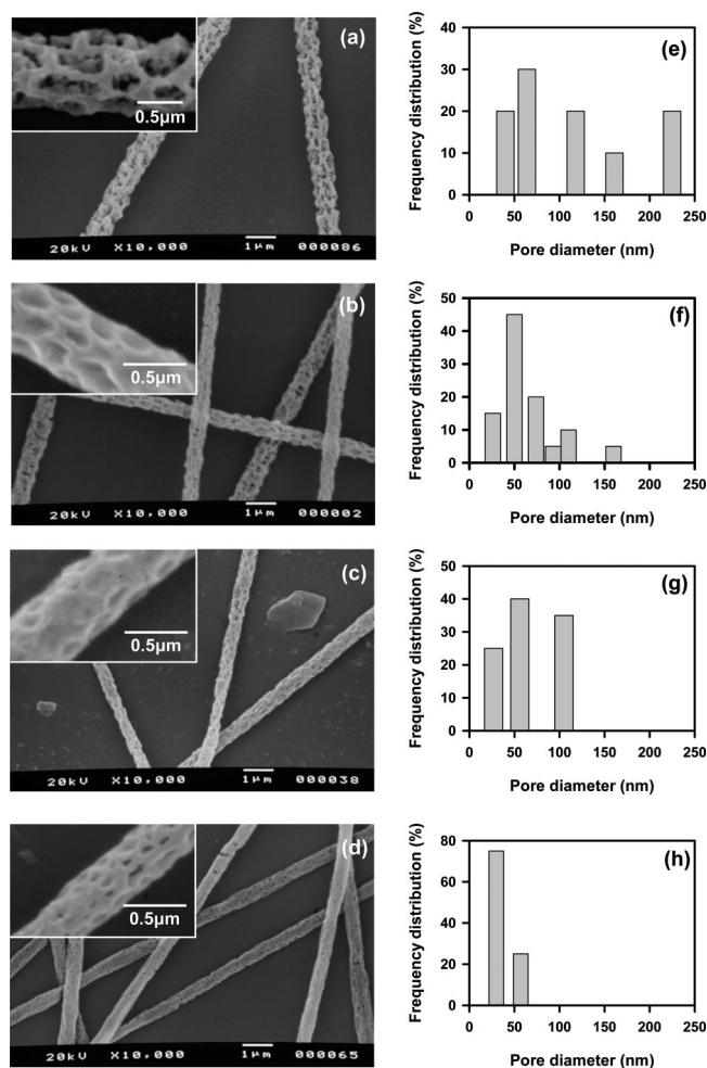
Figure 6. Scanning electron micrographs of the electrospun POM13 nanofibers from an HFIP solution at 55% relative humidity and pore size distributions as a function of electrical voltages: (a, e) for 4 kV, (b, f) for 6 kV, (c, g) for 10 kV, and (d, h) for 15 kV (tip-to-target distance = 10 cm).
