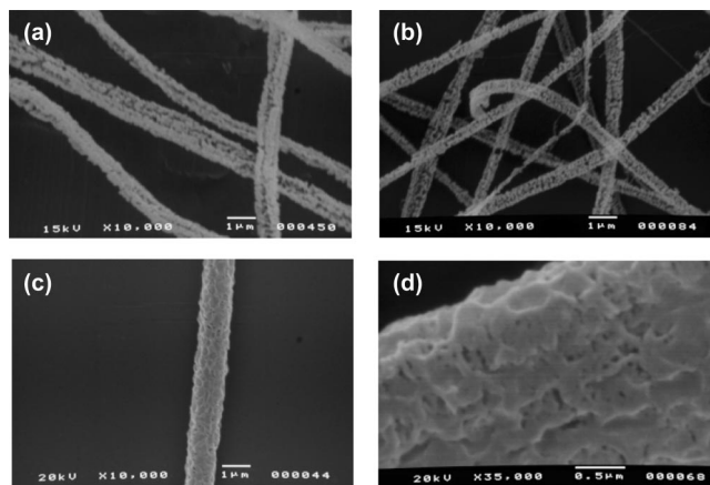
Figure 3. Scanning electron micrographs of the electrospun POM4.4 nanofiber from (a) HFIP/DMF (94:6), (b) HFIP/Glu (90:10), and (c) and (d) HFIP/toluene (70:30) where (d) is magnified to observe the surface morphology of (c) (electrostatic field = 15 kV/10 cm and relative humidity = 75%).
