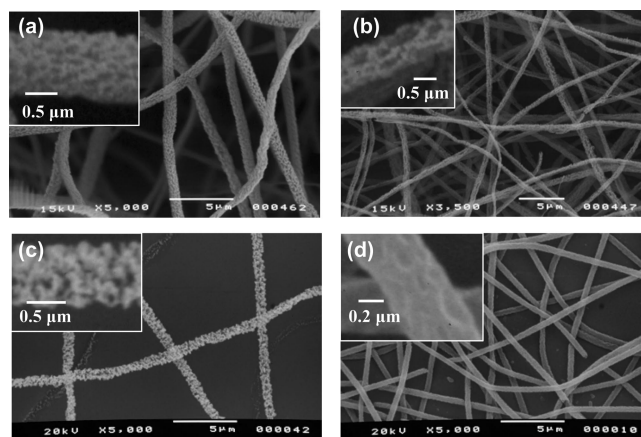
Figure 2. Scanning electron micrographs of the electrospun POM nanofibers from an HFIP solution with copolymer contents of (a) 0, (b) 1.5, (c) 4.4, and (d) 13 wt % (electrostatic field strength = 15 kV/10 cm and relative humidity = 75%).
