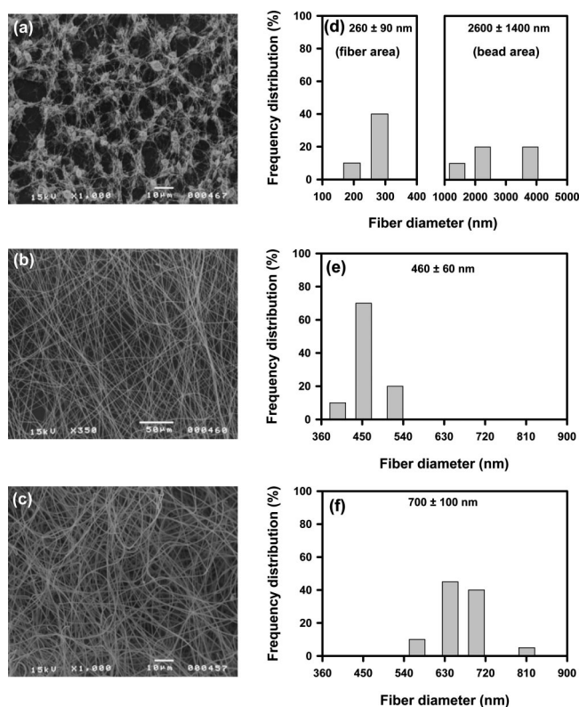
Figure 1. Scanning electron micrographs and frequency distributions of electrospun POM13 nanofibers as a function of polymer concentrations: (a, d) for 3 wt %, (b, e) for 5 wt %, and (c, f) for 10 wt % (electrostatic field strength = 15 kV/10 cm and relative humidity = 75%).
