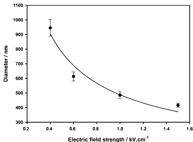
Figure 5. Fiber diameters as a function of electric field strength of electrospun POM13 nanofibers from an HFIP solution (relative humidity = 75%).
